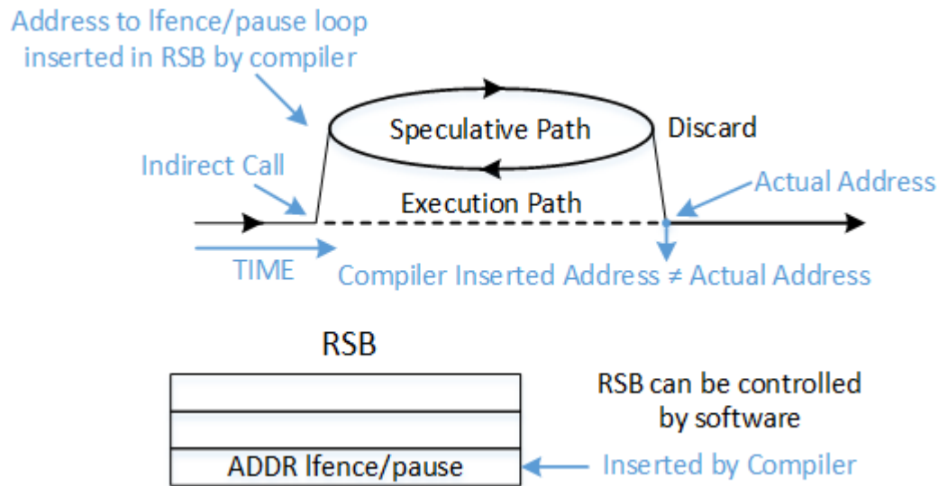
Figure 2: Speculative execution with retpoline
